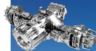
Zero-8 e-Axles
